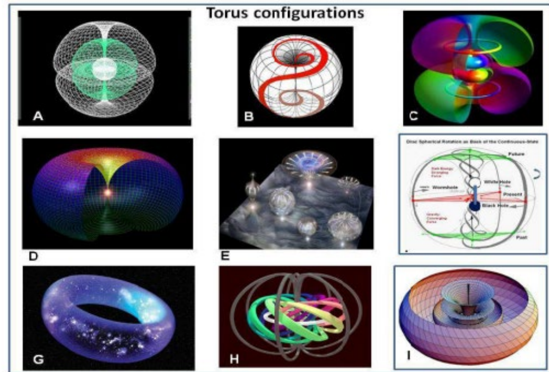
Figure 1. Various modalities of toroidal geometry: A: Nested torus structure B: Torus trajectory (red) C: Atomic structure as double torus, D: Filled space-time structure with singularity, E: Torus network, F: Dirac spherical rotation showing toroidal trajectories in relation to time G: Donut model of the universe, H: Knot structure in torus as metaphor for attractor/standing wave, I: cartoon of a twistor as a supposed space-time unit.
